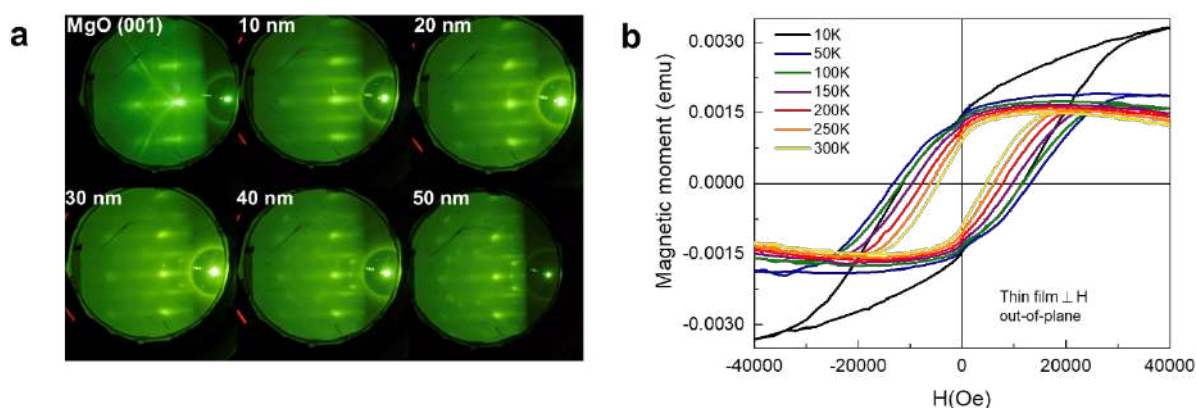
Fig. 1. (a) Evolution of RHEED patterns for 50 nm \text{SmFe}_{12} films epitaxially grown on MgO (001) substrates. (b) Out-of-plane magnetization at different temperatures
